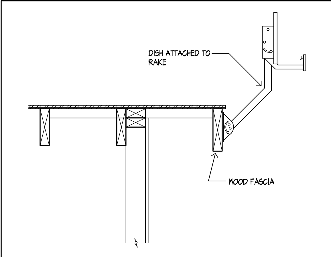
STANDARD RAKE BRACKET
