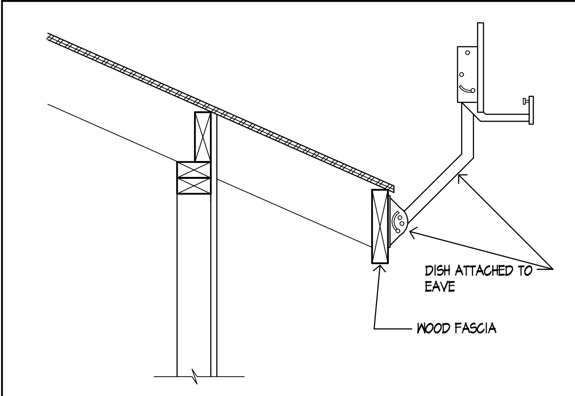
STANDARD EAVE BRACKET
